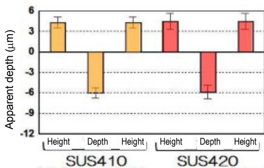
a) White laser marking (3 mm square, 3 × 3 dots)
