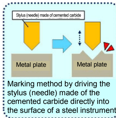
Figure 3. Marking Mechanism of Dot Peen Method
