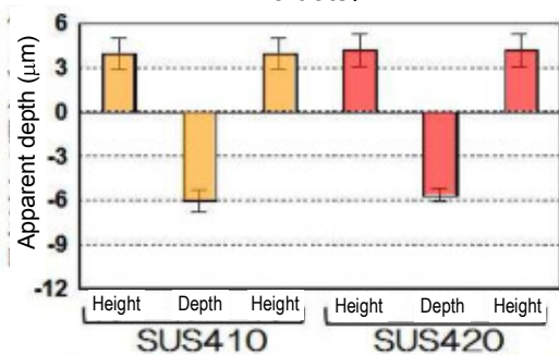
c) White laser marking (5 mm square, 4 × 4 dots)
