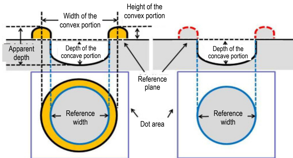
a) Dot shape with an instrument not used b) Dot shape with an instrument worn Figure 6. Cross Section and Upper View of the Dot Formed by Marking
