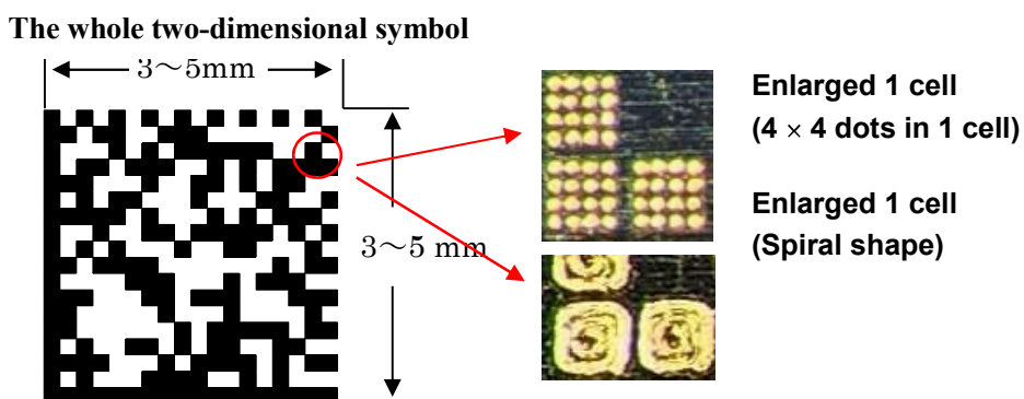
Figure 5. Example of Marking Pattern of Cell
